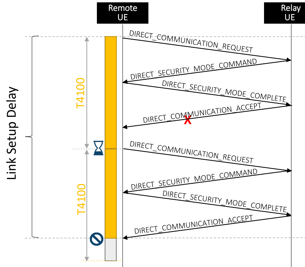
Direct Communication Link Setup Procedure
